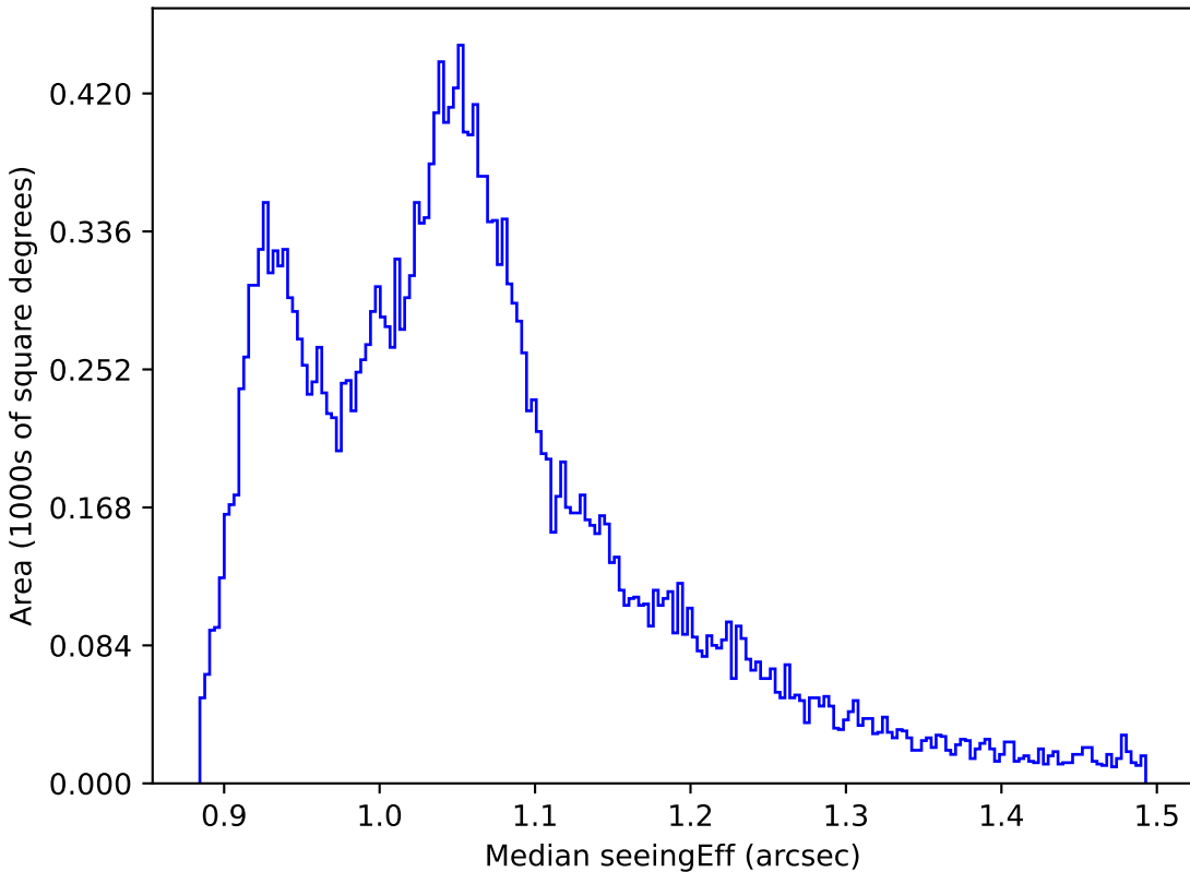
mw_roll_all_v3.3_10yrs All sky all bands: Median seeingEff
