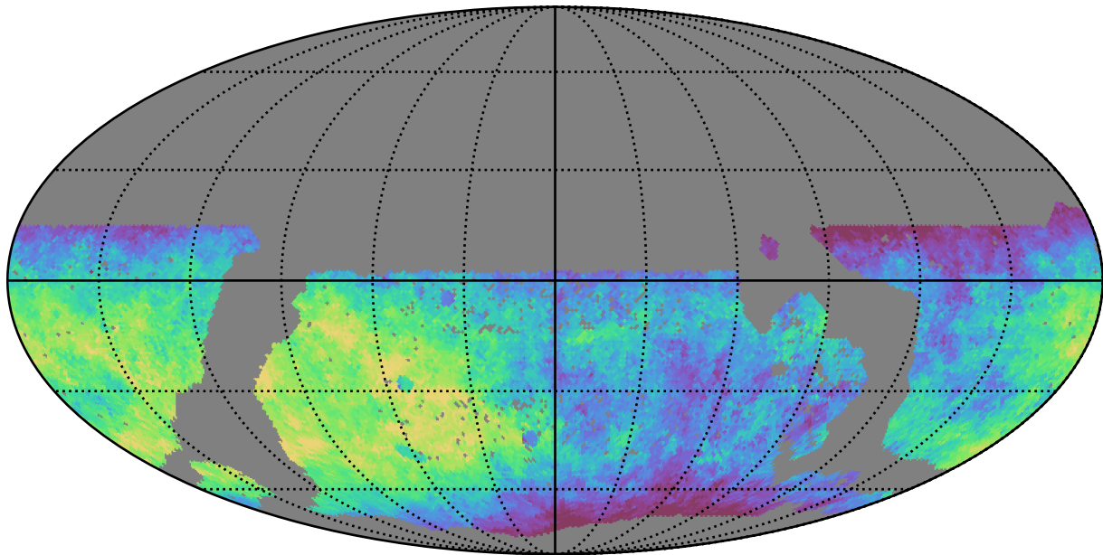
mw_roll_all_v3.3_10yrs WFD z band: Median saturation_mag
