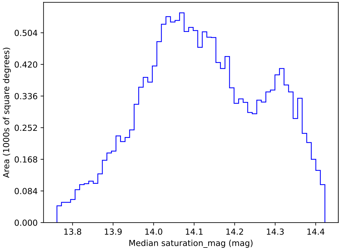
mw_roll_all_v3.3_10yrs WFD z band: Median saturation_mag
