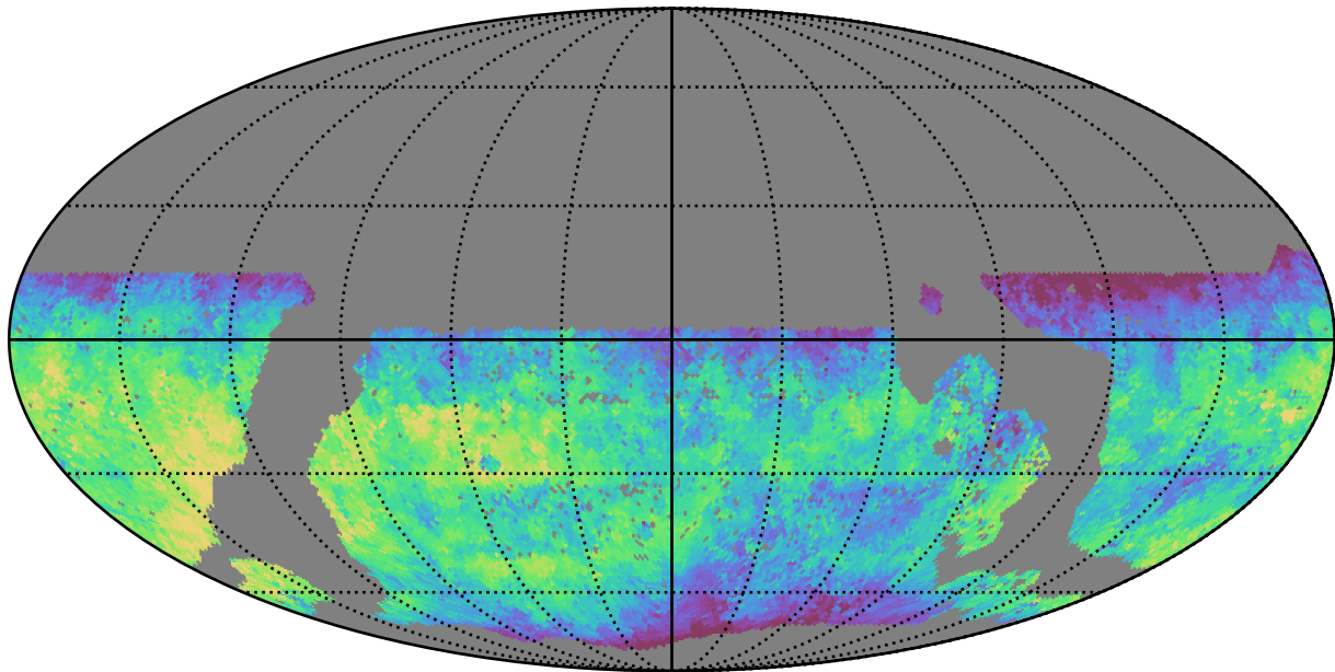
mw_roll_all_v3.3_10yrs WFD u band: Median saturation_mag
