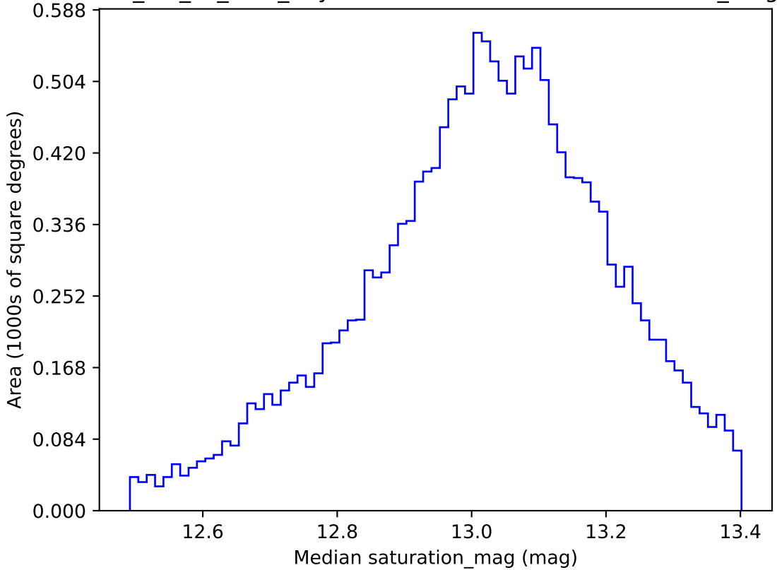
mw_roll_all_v3.3_10yrs WFD u band: Median saturation_mag
