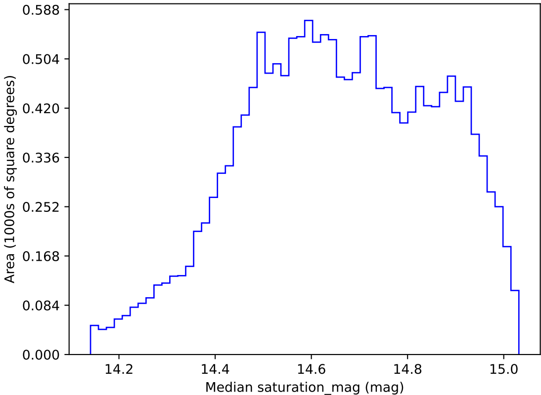
mw_roll_all_v3.3_10yrs WFD r band: Median saturation_mag
