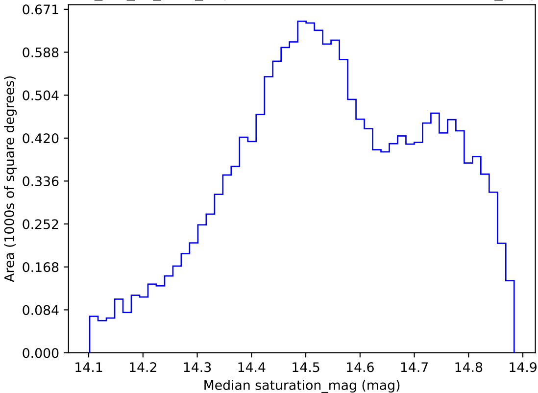
mw_roll_all_v3.3_10yrs WFD i band: Median saturation_mag
