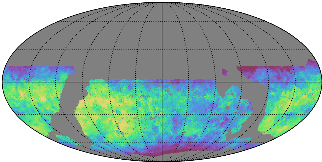
mw_roll_all_v3.3_10yrs WFD g band: Median saturation_mag
