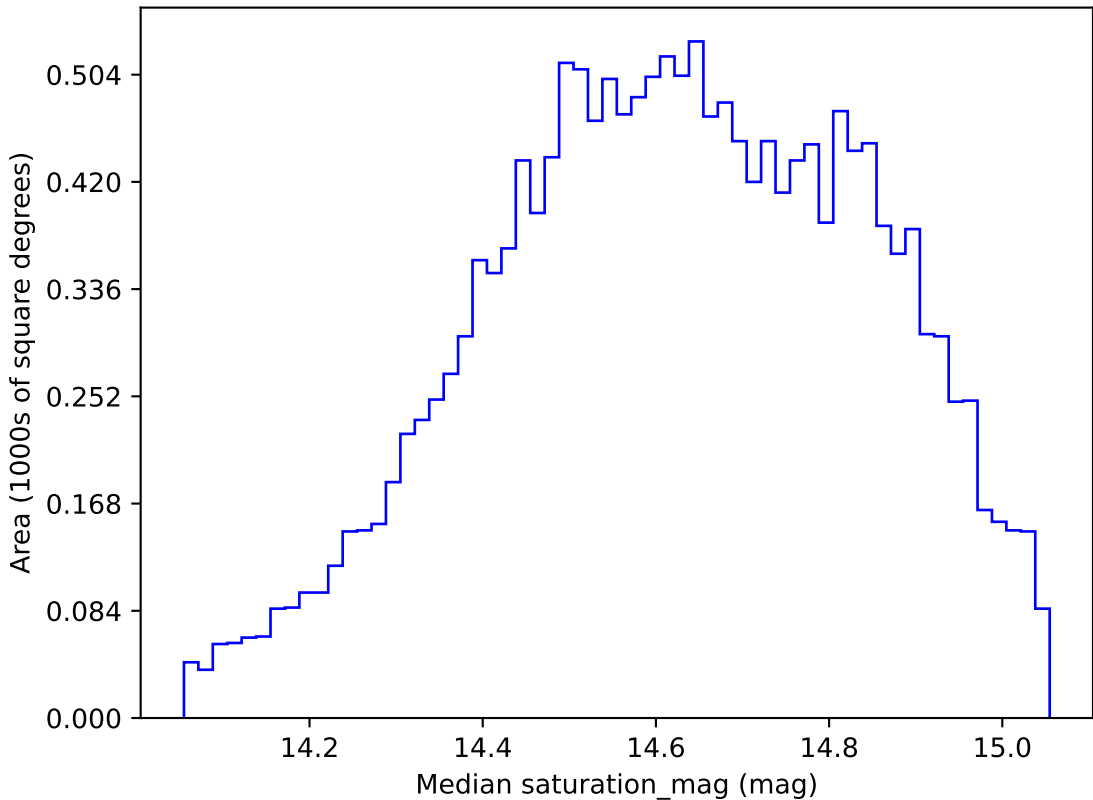
mw_roll_all_v3.3_10yrs WFD g band: Median saturation_mag
