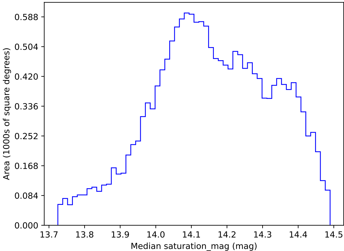
mw_roll_all_v3.3_10yrs WFD all bands: Median saturation_mag
