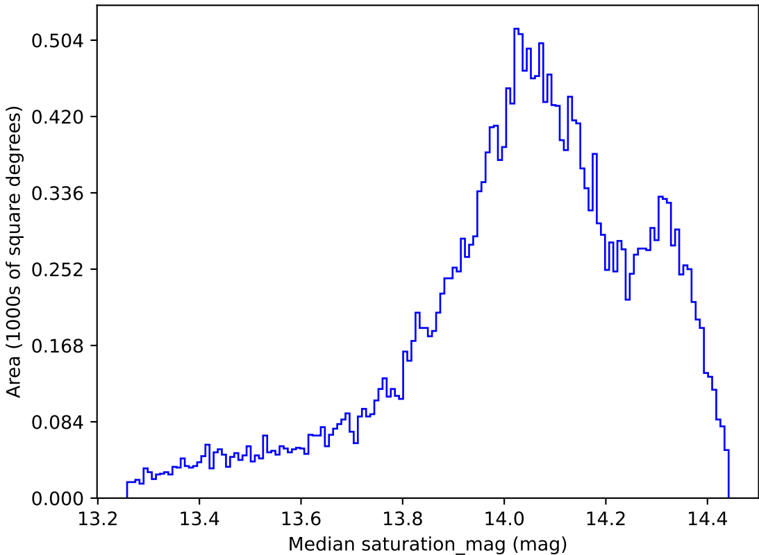
mw_roll_all_v3.3_10yrs All sky z band: Median saturation_mag
