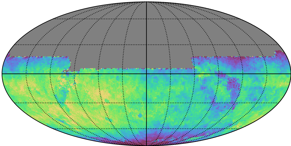
mw_roll_all_v3.3_10yrs All sky y band: Median saturation_mag
