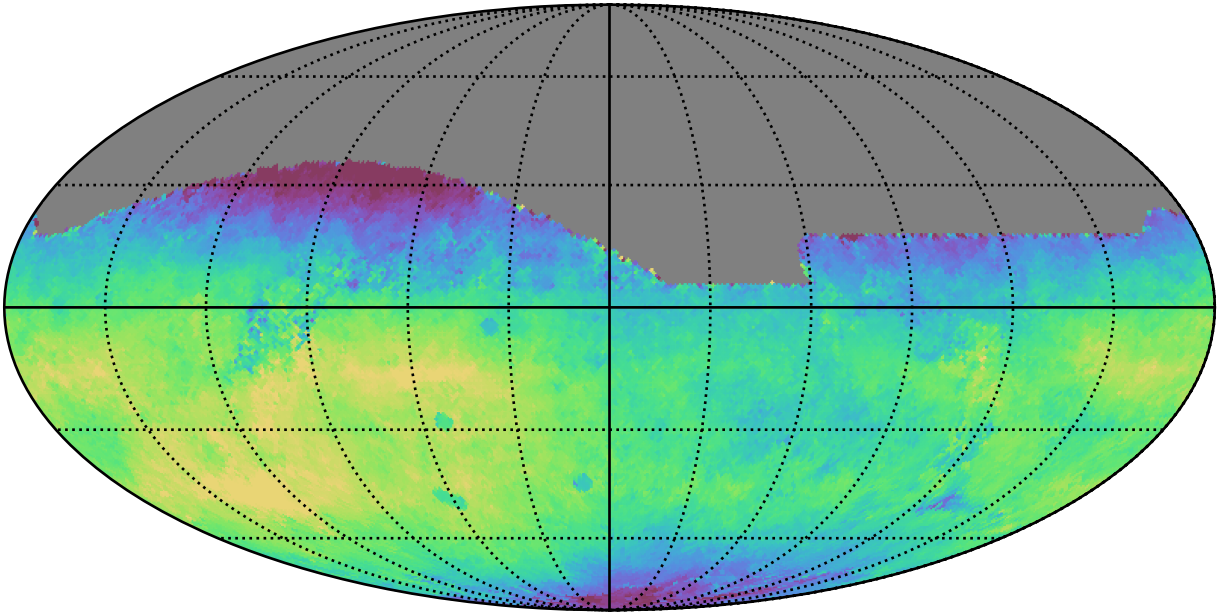
mw_roll_all_v3.3_10yrs All sky r band: Median saturation_mag
