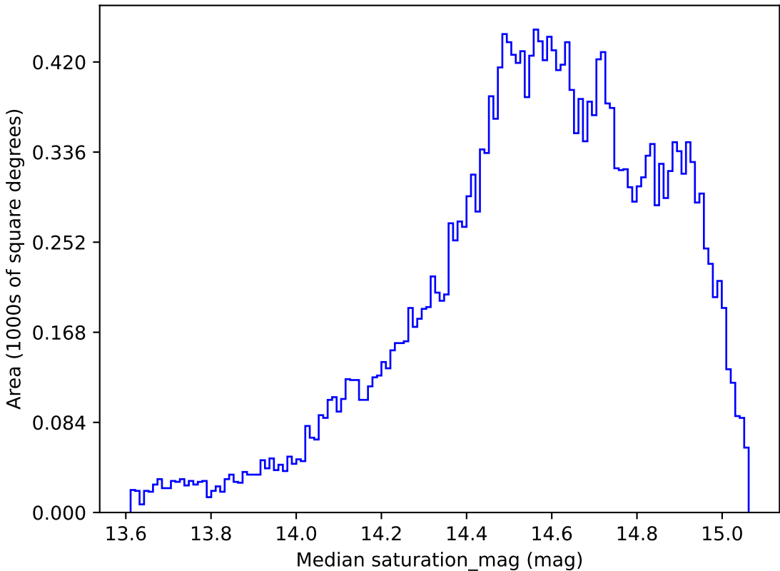
mw_roll_all_v3.3_10yrs All sky r band: Median saturation_mag
