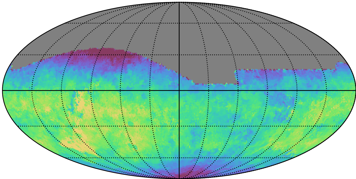
mw_roll_all_v3.3_10yrs All sky g band: Median saturation_mag
