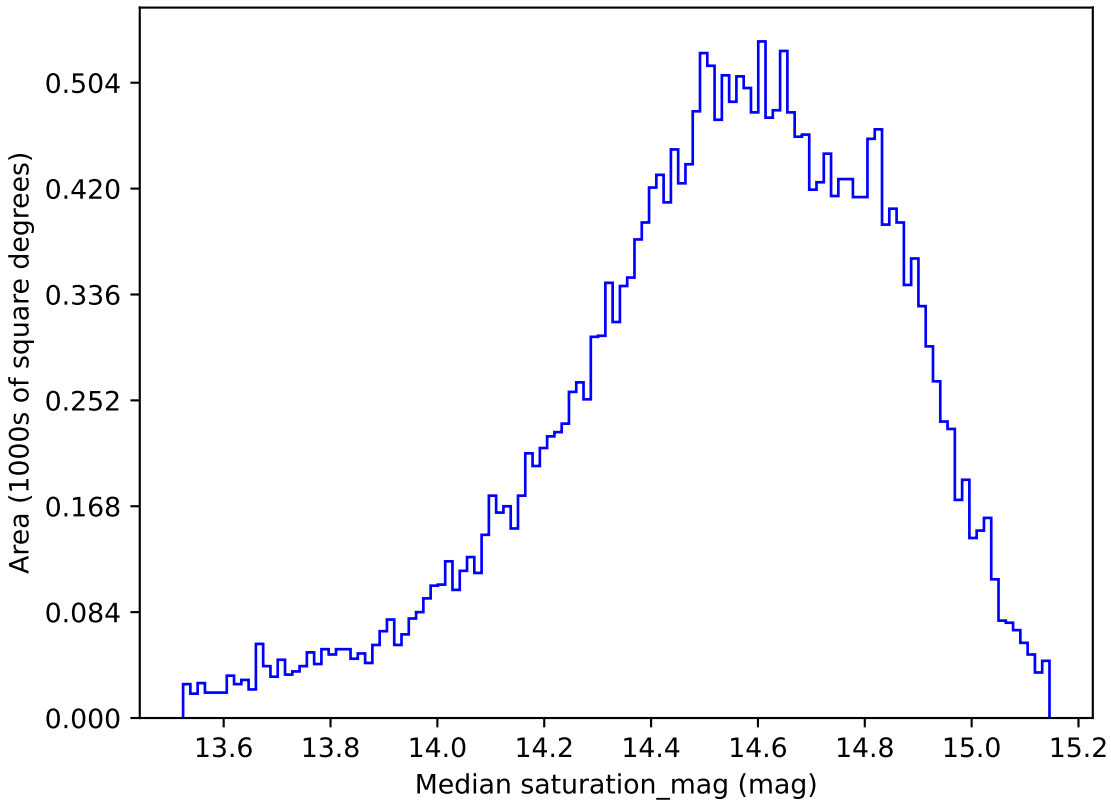
mw_roll_all_v3.3_10yrs All sky g band: Median saturation_mag
