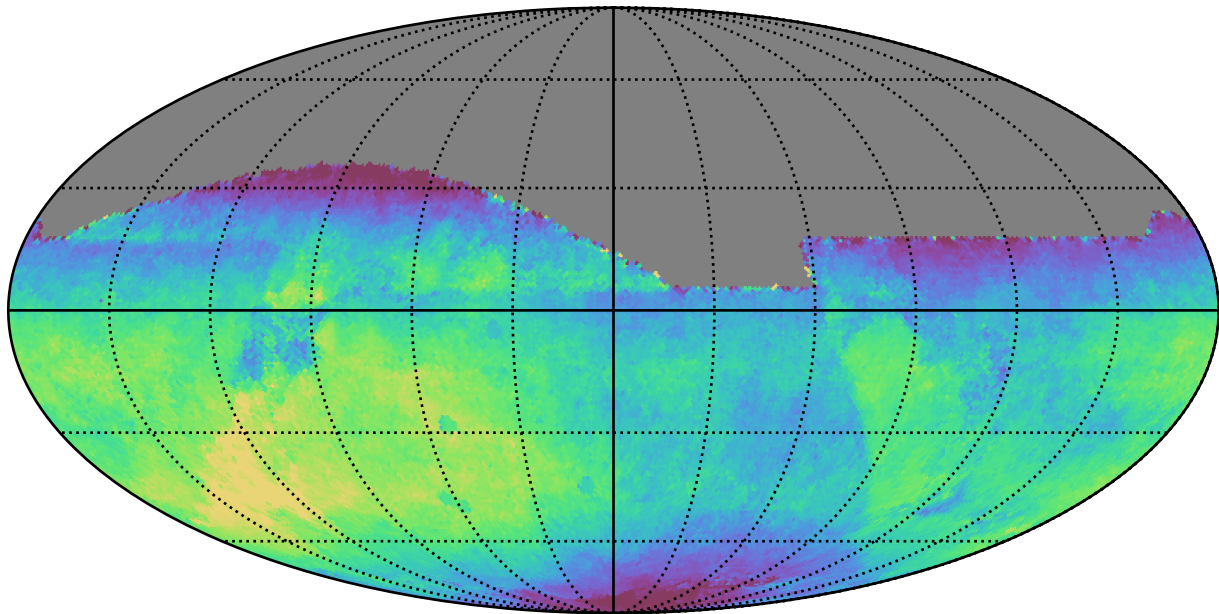
mw_roll_all_v3.3_10yrs All sky all bands: Median saturation_mag
