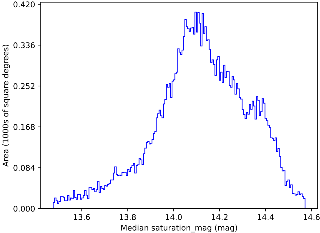
mw_roll_all_v3.3_10yrs All sky all bands: Median saturation_mag
