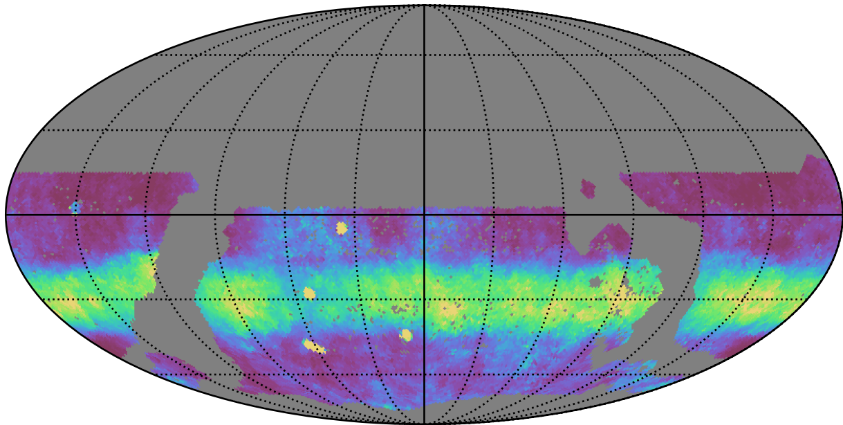
mw_roll_all_v3.3_10yrs WFD z band: Median normairmass
