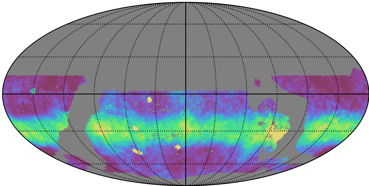
mw_roll_all_v3.3_10yrs WFD y band: Median normairmass
