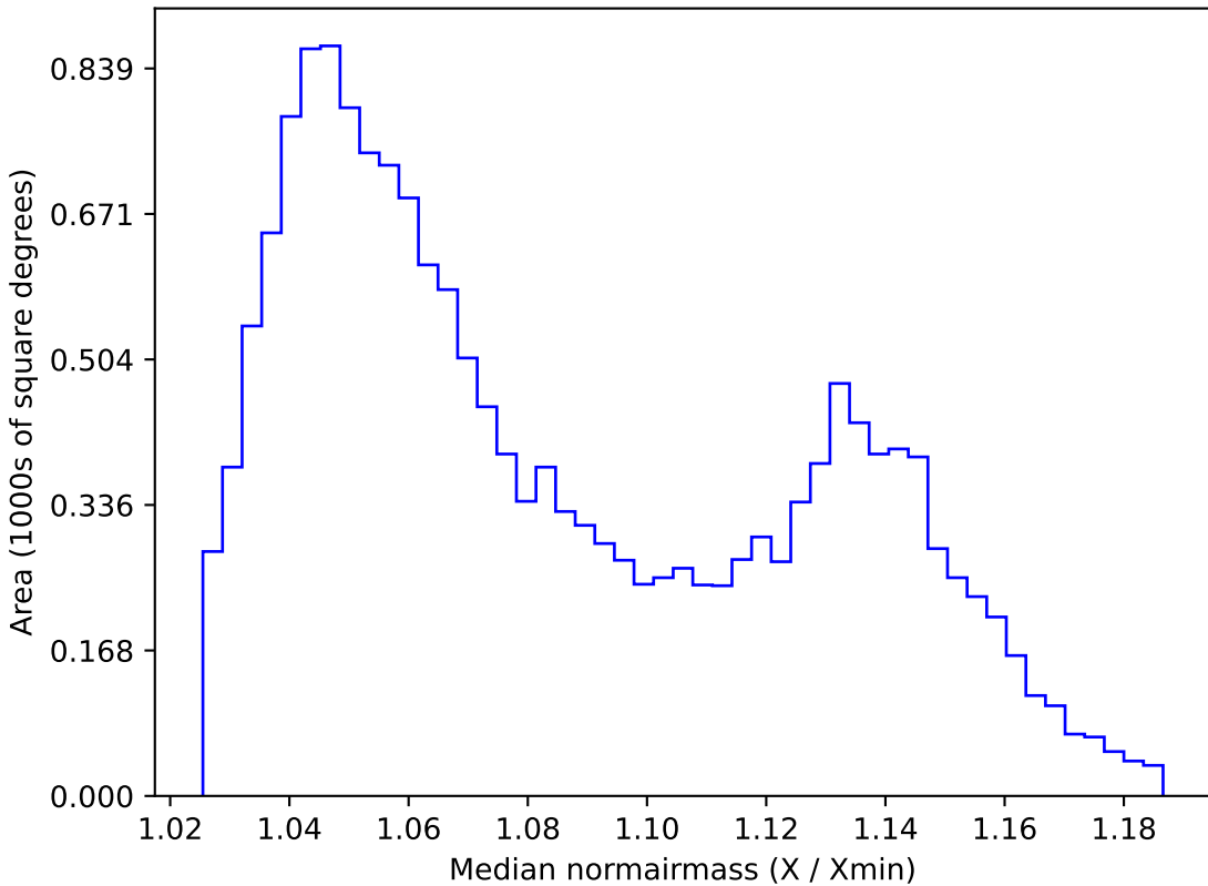
mw_roll_all_v3.3_10yrs WFD y band: Median normairmass
