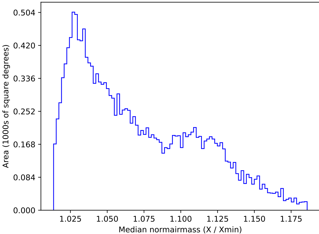
mw_roll_all_v3.3_10yrs WFD u band: Median normairmass
