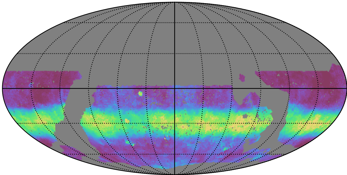
mw_roll_all_v3.3_10yrs WFD i band: Median normairmass
