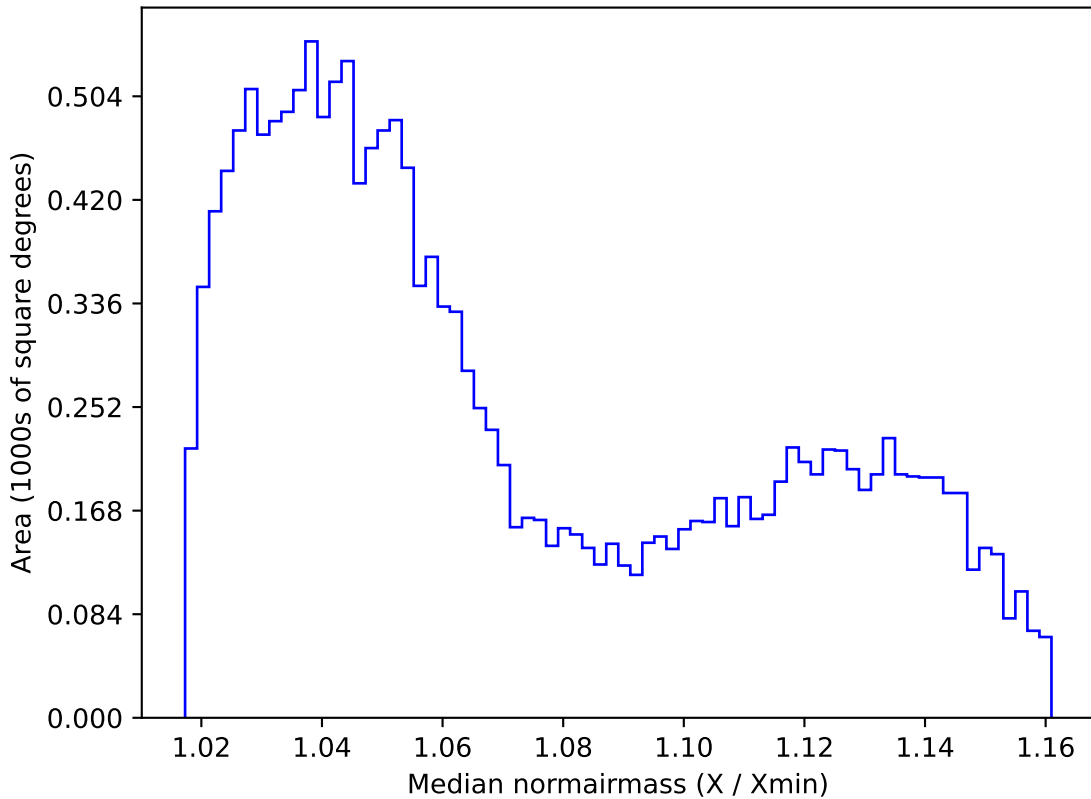
mw_roll_all_v3.3_10yrs WFD i band: Median normairmass
