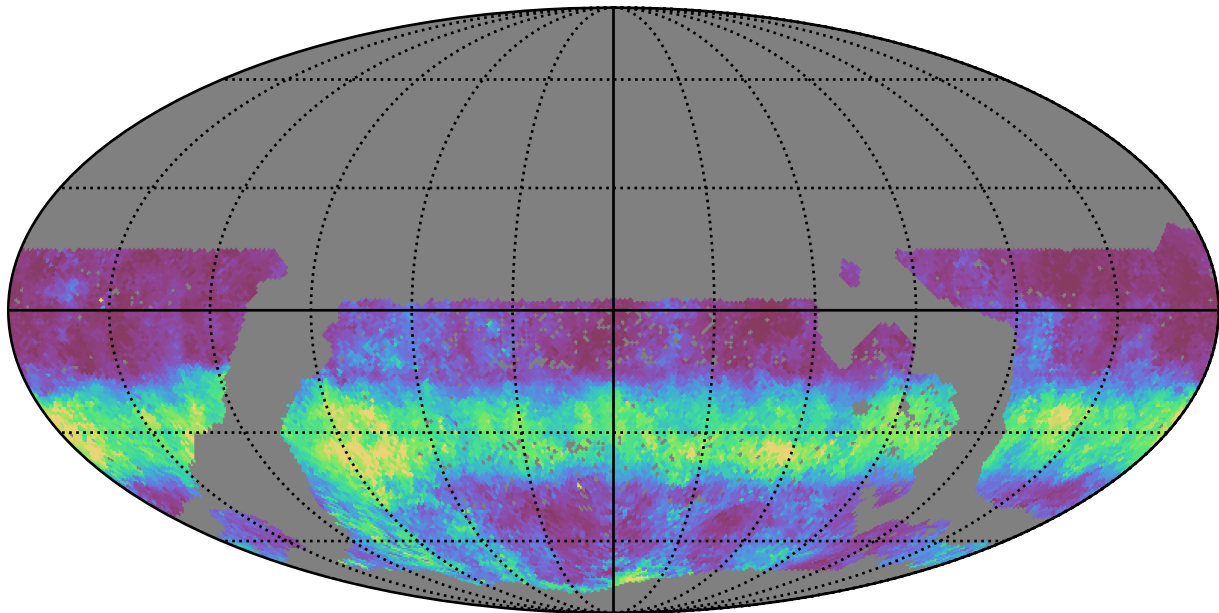
mw_roll_all_v3.3_10yrs WFD g band: Median normairmass
