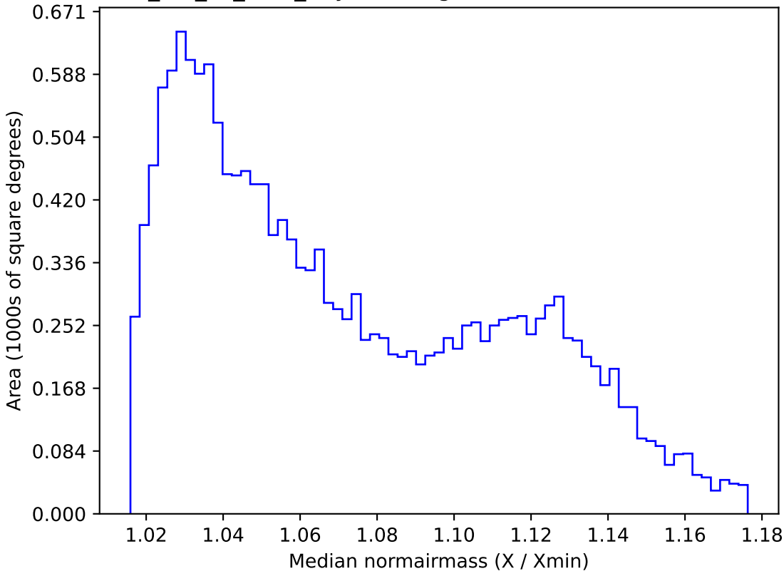
mw_roll_all_v3.3_10yrs WFD g band: Median normairmass
