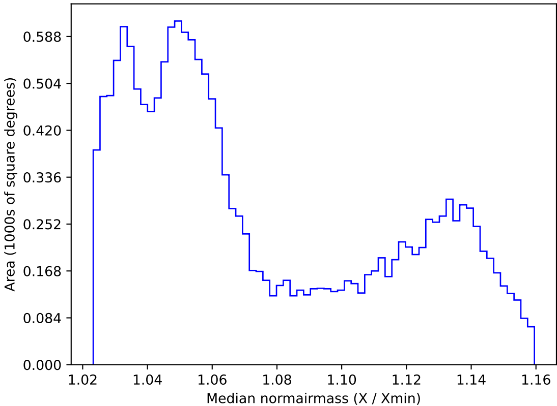
mw_roll_all_v3.3_10yrs WFD all bands: Median normairmass
