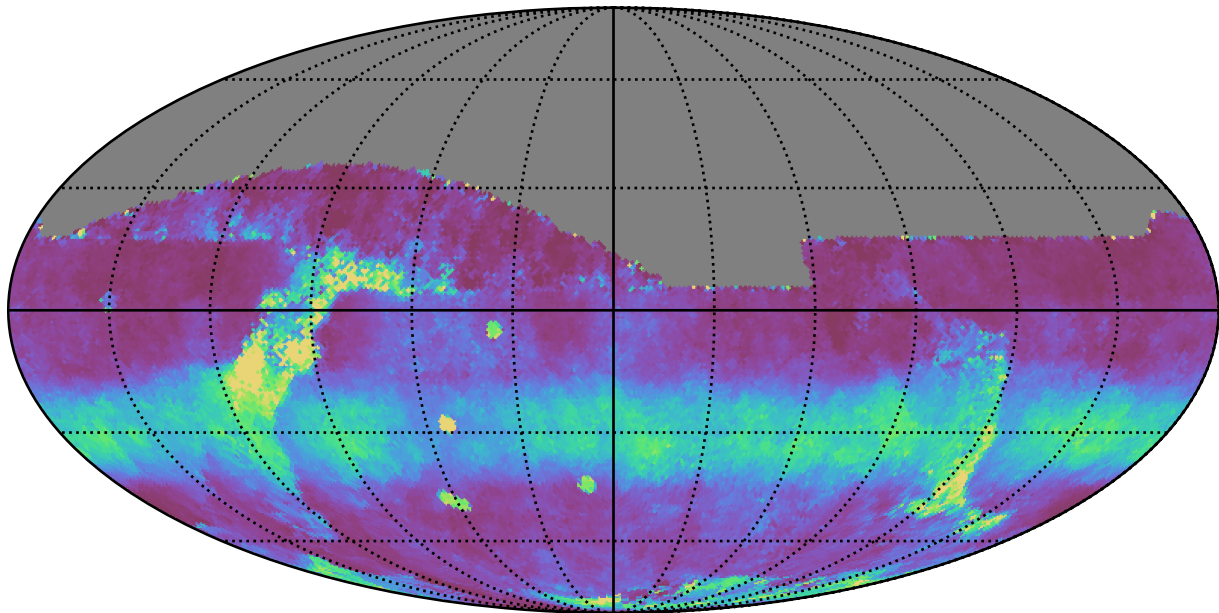
mw_roll_all_v3.3_10yrs All sky z band: Median normairmass
