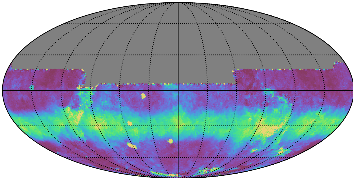
mw_roll_all_v3.3_10yrs All sky y band: Median normairmass
