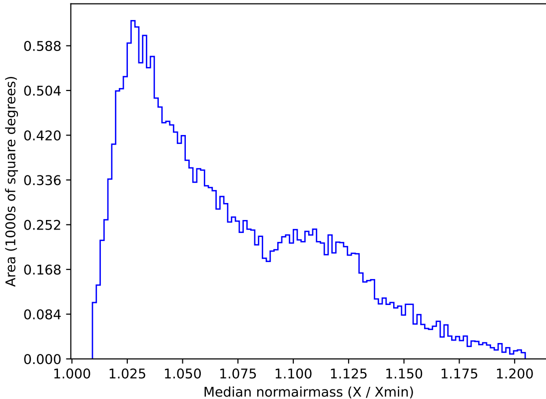
mw_roll_all_v3.3_10yrs All sky u band: Median normairmass
