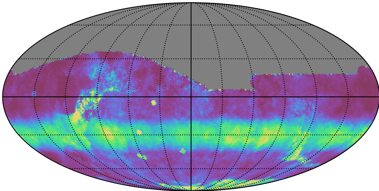
mw_roll_all_v3.3_10yrs All sky r band: Median normairmass
