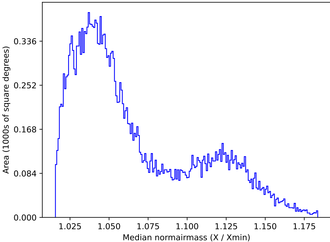
mw_roll_all_v3.3_10yrs All sky r band: Median normairmass
