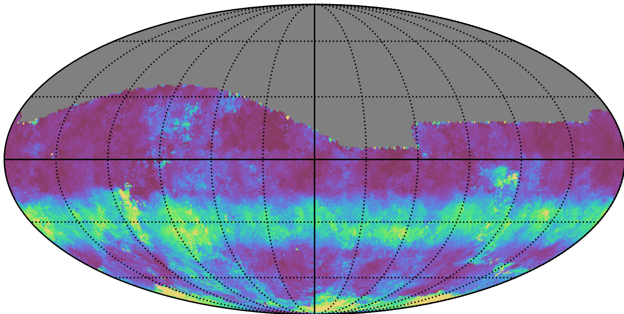
mw_roll_all_v3.3_10yrs All sky g band: Median normairmass
