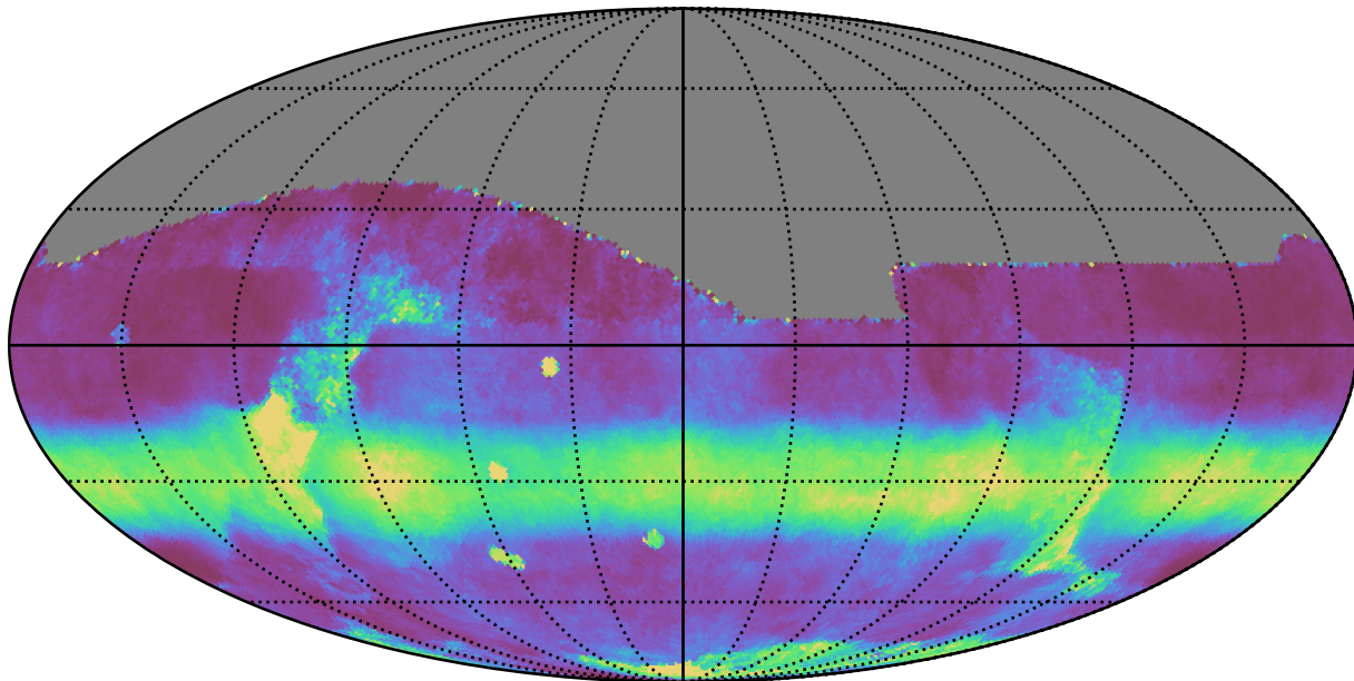
mw_roll_all_v3.3_10yrs All sky all bands: Median normairmass
