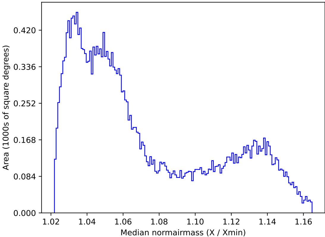
mw_roll_all_v3.3_10yrs All sky all bands: Median normairmass
