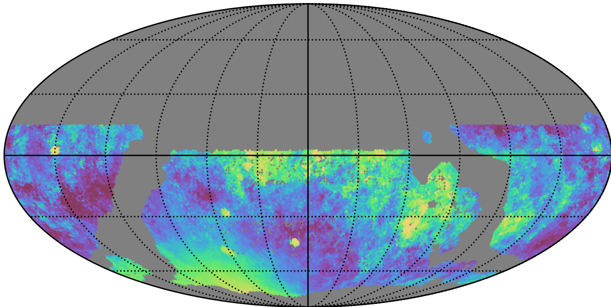
mw_roll_all_v3.3_10yrs WFD z band: Median moonDistance
