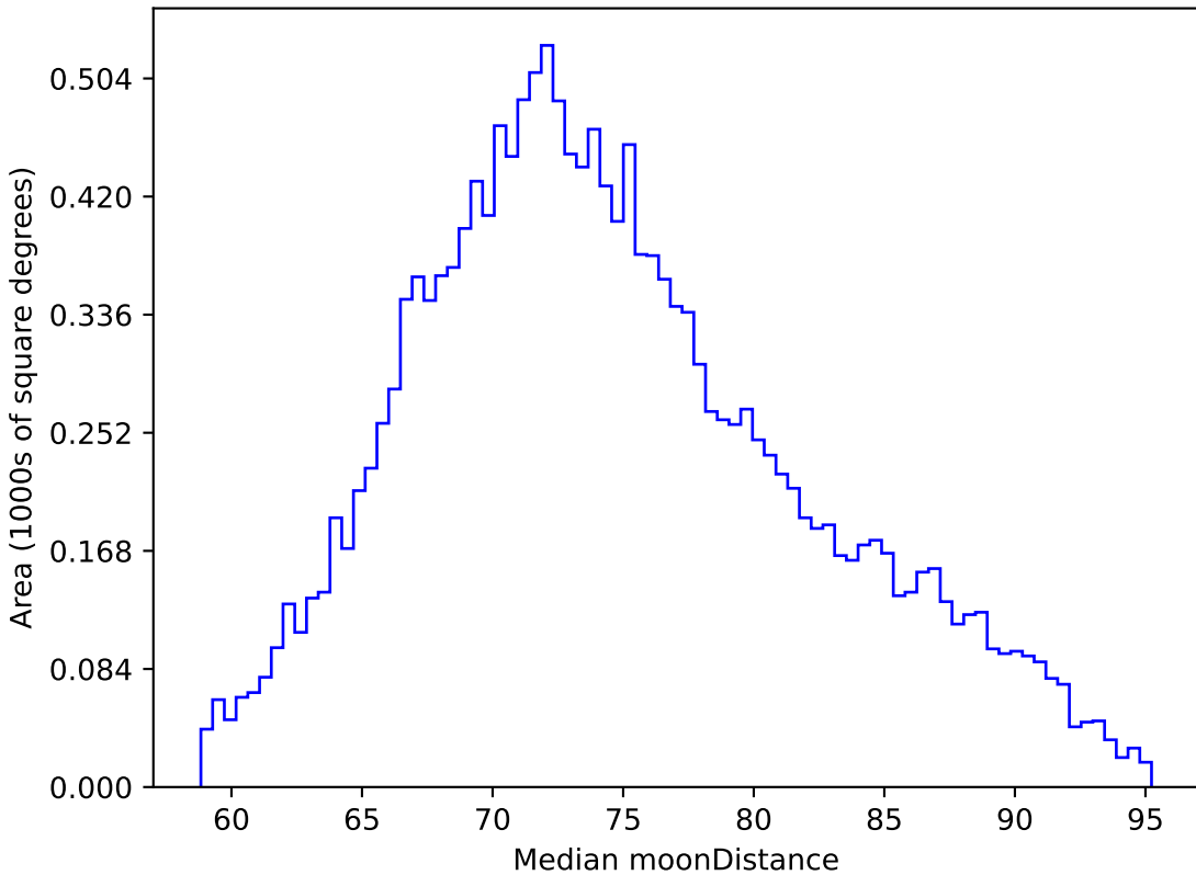
mw_roll_all_v3.3_10yrs WFD z band: Median moonDistance
