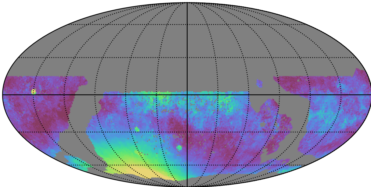
mw_roll_all_v3.3_10yrs WFD y band: Median moonDistance
