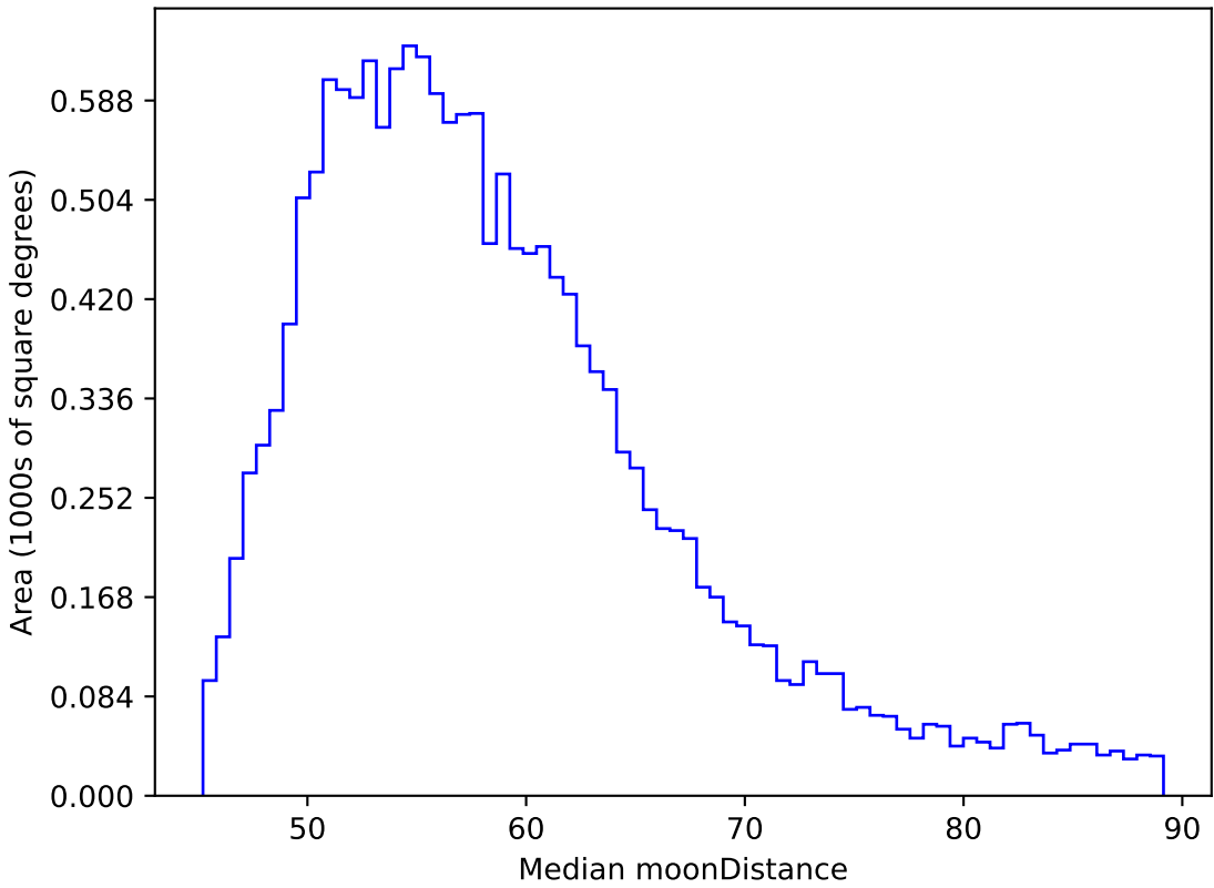
mw_roll_all_v3.3_10yrs WFD y band: Median moonDistance
