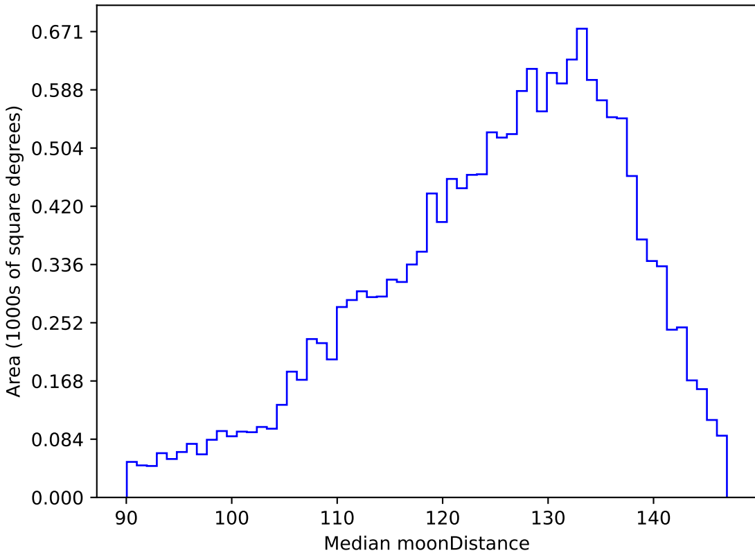
mw_roll_all_v3.3_10yrs WFD u band: Median moonDistance
