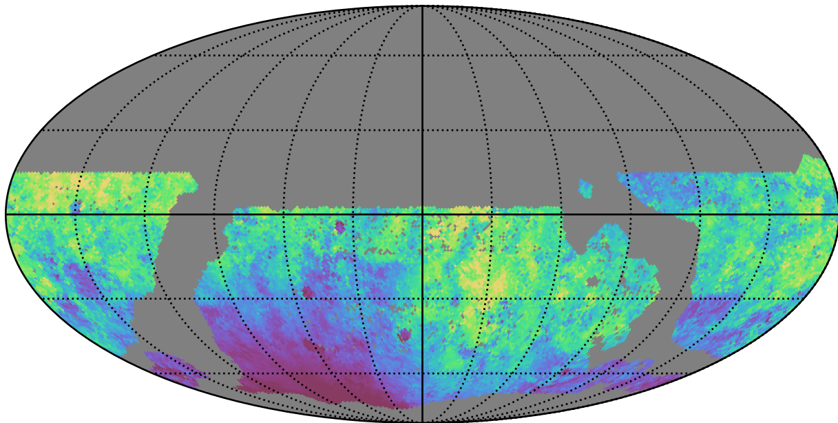
mw_roll_all_v3.3_10yrs WFD r band: Median moonDistance
