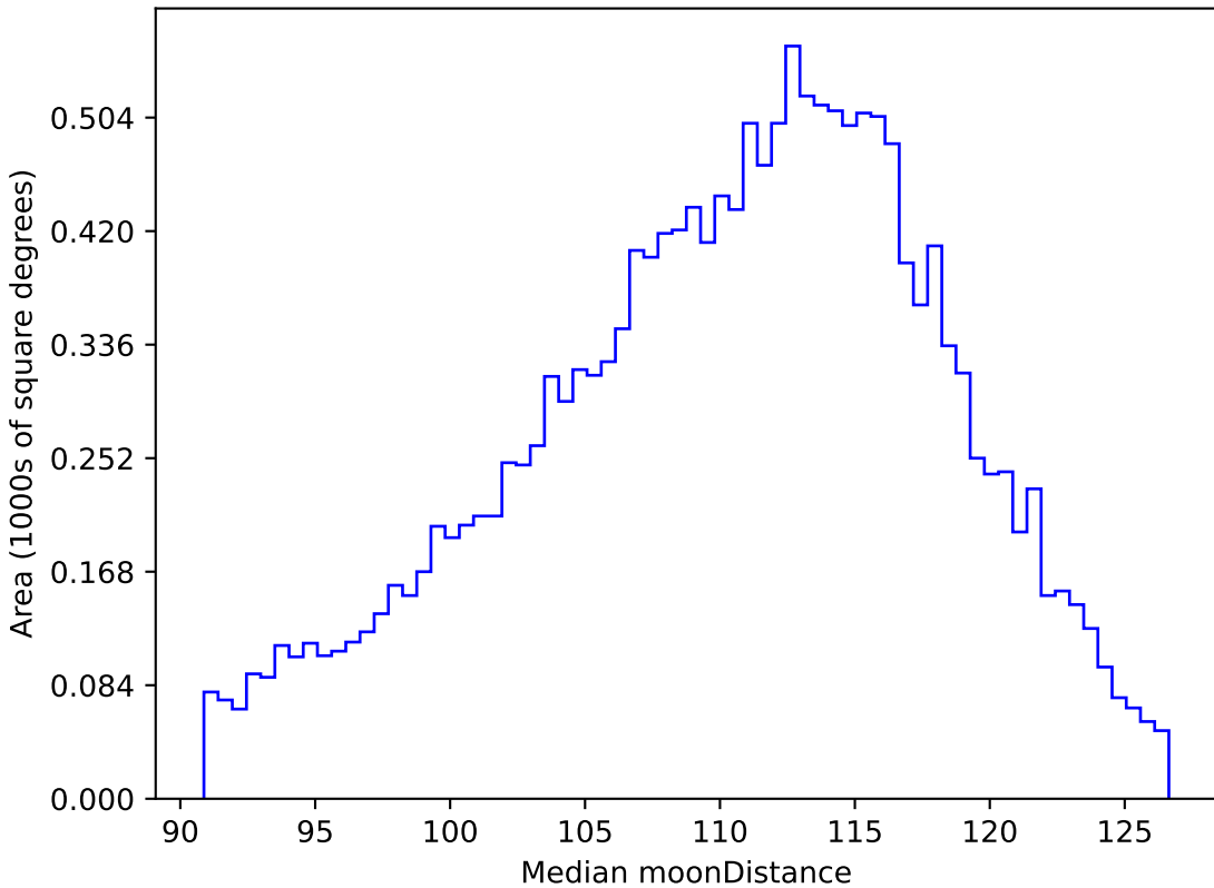
mw_roll_all_v3.3_10yrs WFD r band: Median moonDistance
