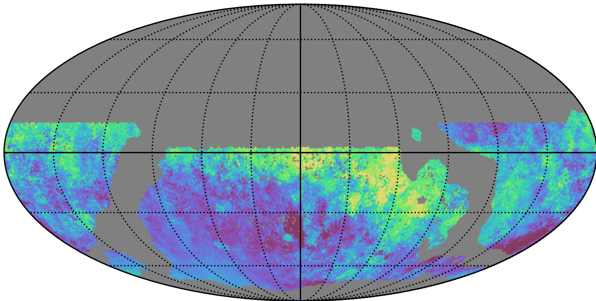
mw_roll_all_v3.3_10yrs WFD i band: Median moonDistance
