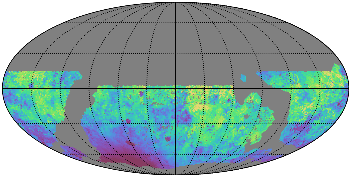
mw_roll_all_v3.3_10yrs WFD g band: Median moonDistance
