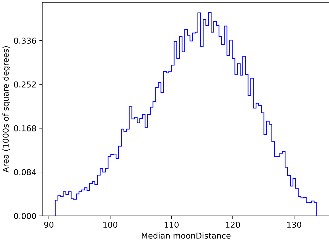
mw_roll_all_v3.3_10yrs WFD g band: Median moonDistance
