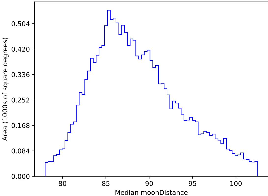
mw_roll_all_v3.3_10yrs WFD all bands: Median moonDistance
