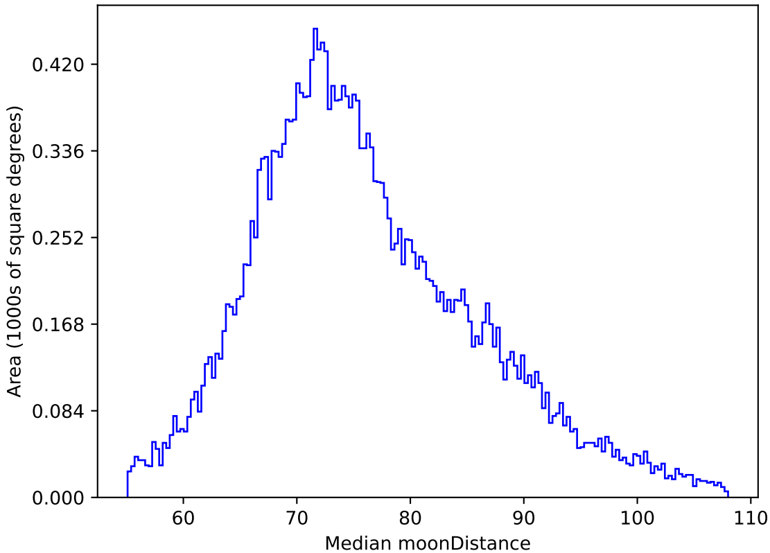
mw_roll_all_v3.3_10yrs All sky z band: Median moonDistance
