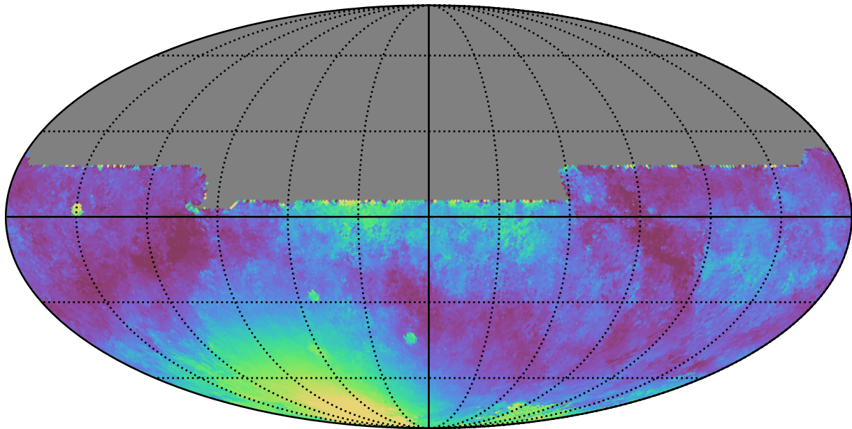
mw_roll_all_v3.3_10yrs All sky y band: Median moonDistance
