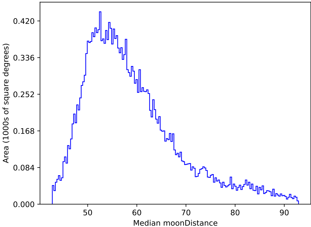
mw_roll_all_v3.3_10yrs All sky y band: Median moonDistance
