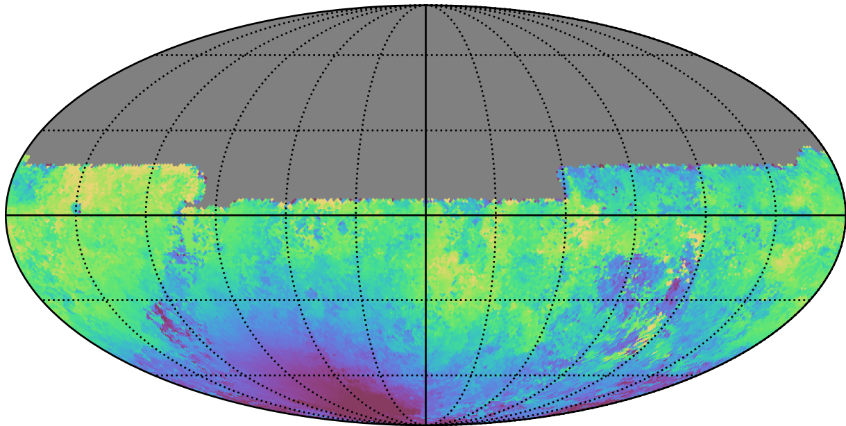
mw_roll_all_v3.3_10yrs All sky u band: Median moonDistance
